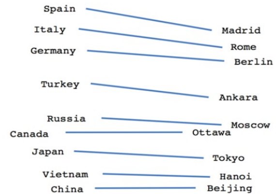
Country-Capital
