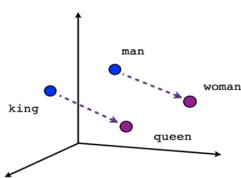
Male-Female
