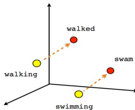
Verb tense
